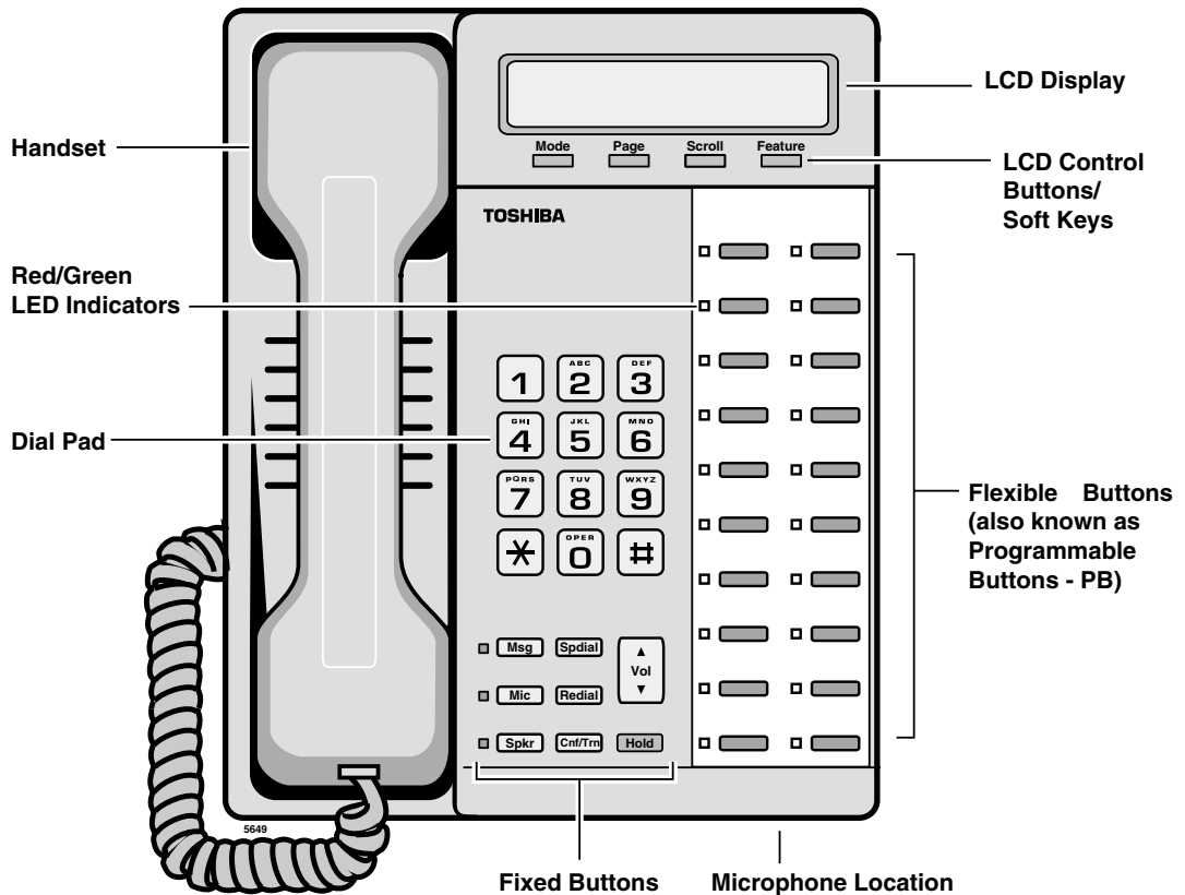
DKT3020-SD Telephone
